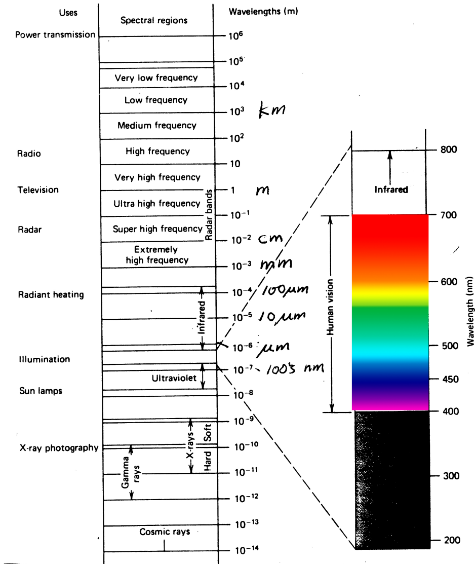
Electromagnetic spectrum, showing the position of the visible region in relation to other regions. The boundaries between regions are indicated by wavelengths measured in vacuum.
