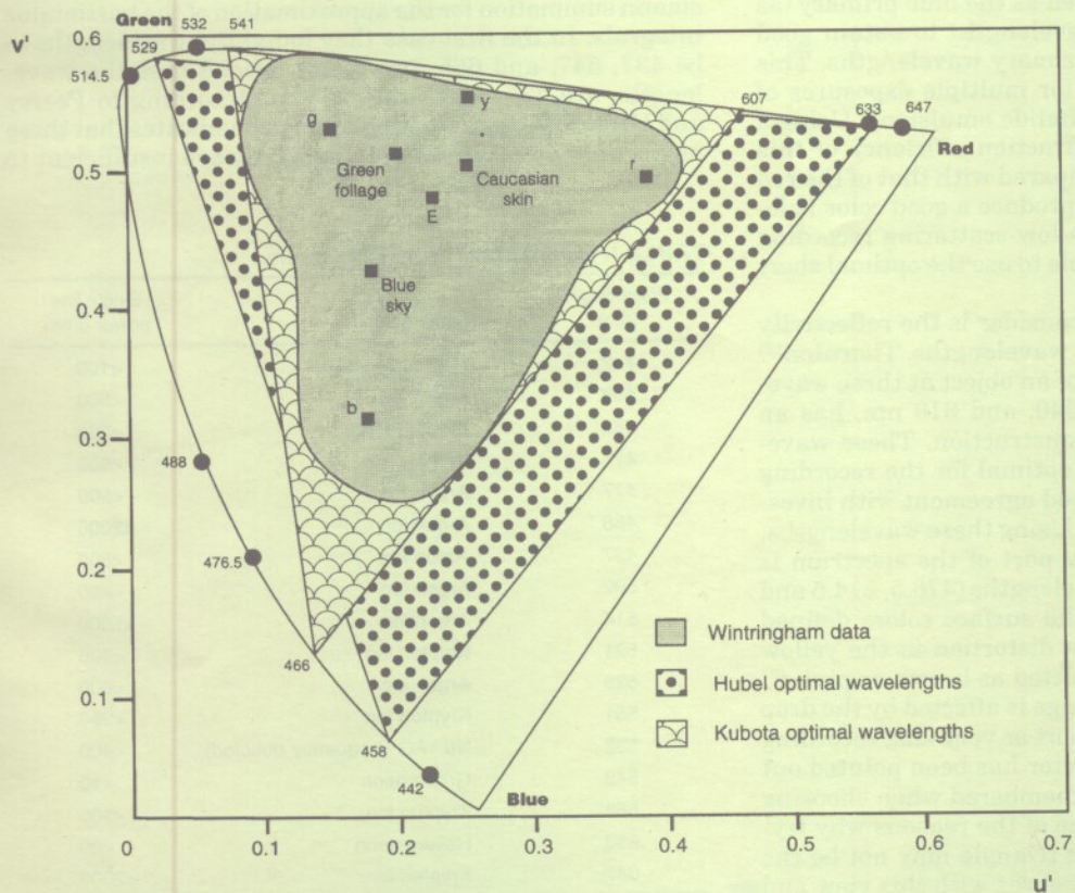
Figure 3. The 1976 CIE uniform scales chromaticity diagram shows the gamut of surface colors and positions of common laser wavelengths. Hubel's and Kubota's three optimal color-recording laser wavelengths are also indicated.
