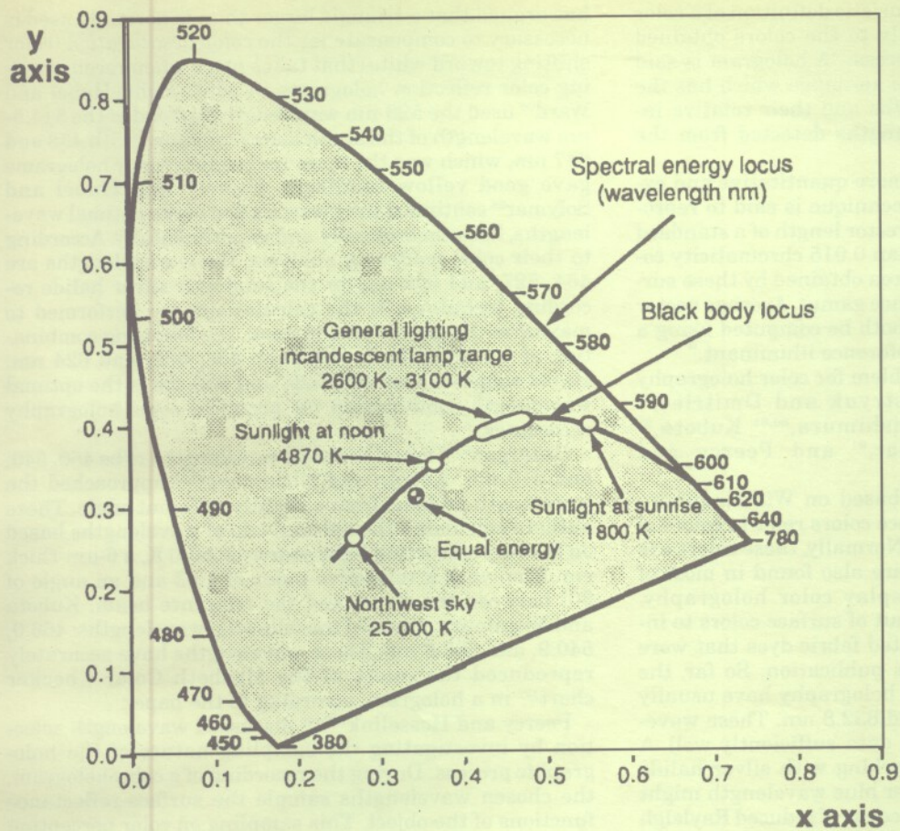
Figure 2. The 1931 CIE chromaticity diagram, illustrating the chromaticities of various light sources.
