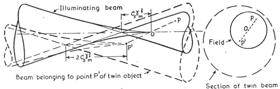
FIGURE 9. The twin object in a beam with spherical aberration.
