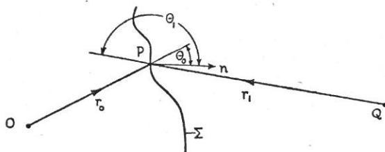
FIGURE 2. Fresnel-Kirchhoff diffraction formula.
