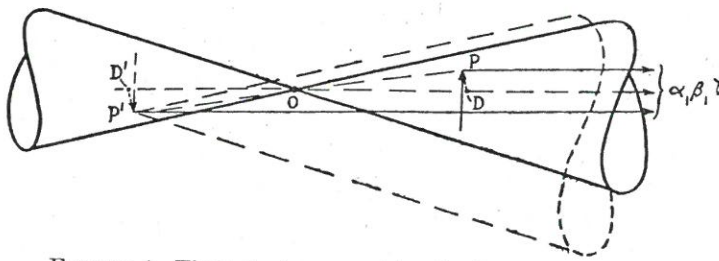
FIGURE 4. The twin images arising in the reconstruction.
